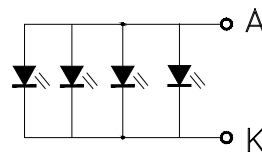
Backlight Circuit Diagram: (背光电路图)
