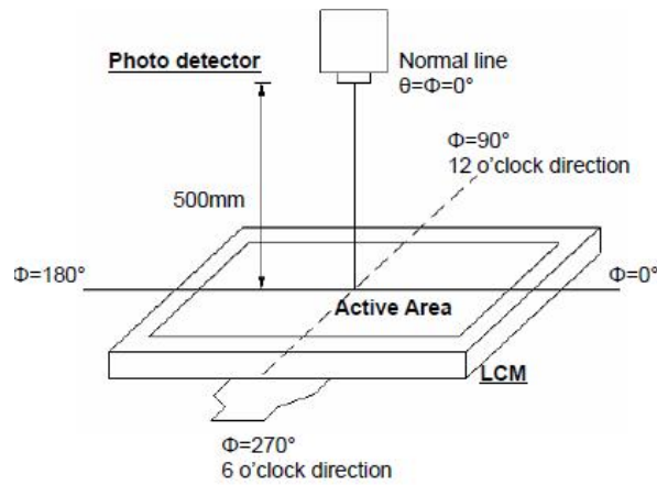
Fig. 4-2 Optical measurement system setup
