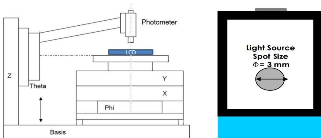
FIG. 1 DMS-803 Measurement Set-Up
